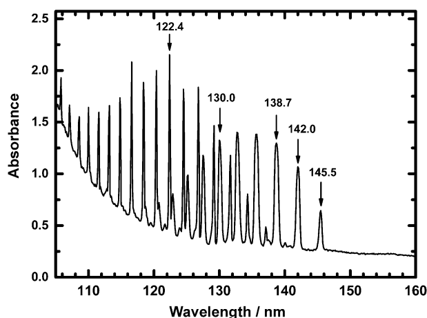
Figure 1. Absorption spectrum (resolution 0.1\text{ nm} , step 0.1\text{ nm} ) of pure solid nitrogen at 3 K in the wavelength range 105\text{--}160\text{ nm} . The thickness of the nitrogen film is estimated to be 8\text{--}10\text{ }\mu\text{m} .
