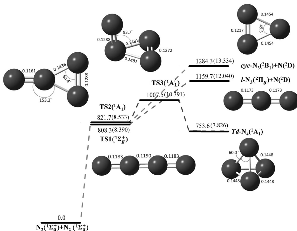
Figure 3. Energies [ \text{kJ mol}^{-1} , eV in parentheses] along reaction paths for the reaction N_2 + N_2 . The energies calculated at the stationary points are indicated in the figure. The calculated geometries (bond lengths [nm], angles [ ^\circ ]) of TS1, TS2, TS3, \text{cyc-N}_3 , \text{l-N}_3 , and \text{Td-N}_4 are displayed. The structures were optimized with B3LYP/aug-cc-pVTZ; their energies were calculated with basis set CCSD(T)/aug-cc-pVTZ.
